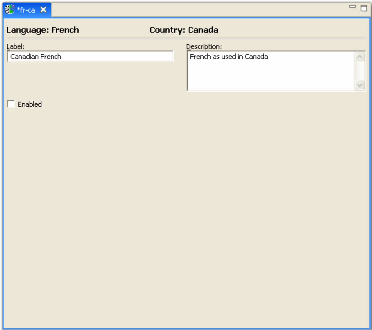
Figure 4: Locale Editor
