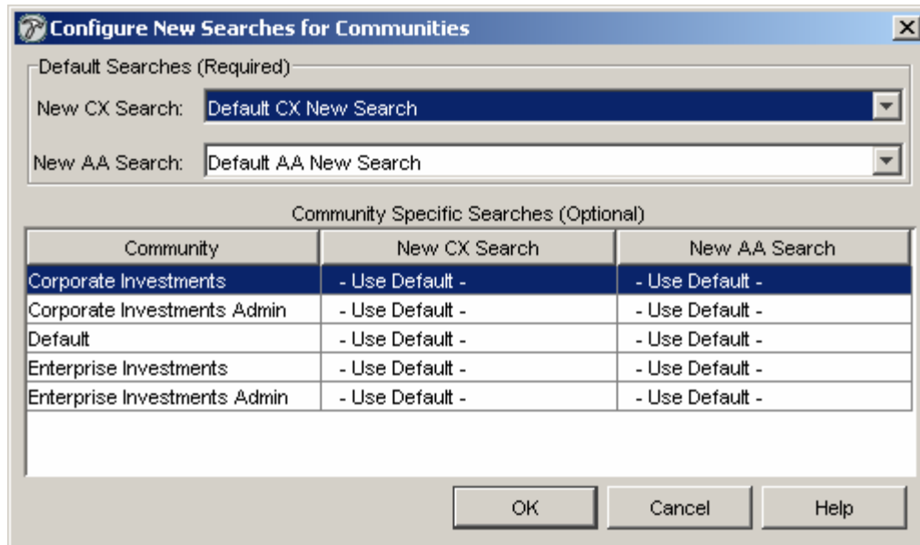
Figure 25: Configure New Searches for Communities dialog
