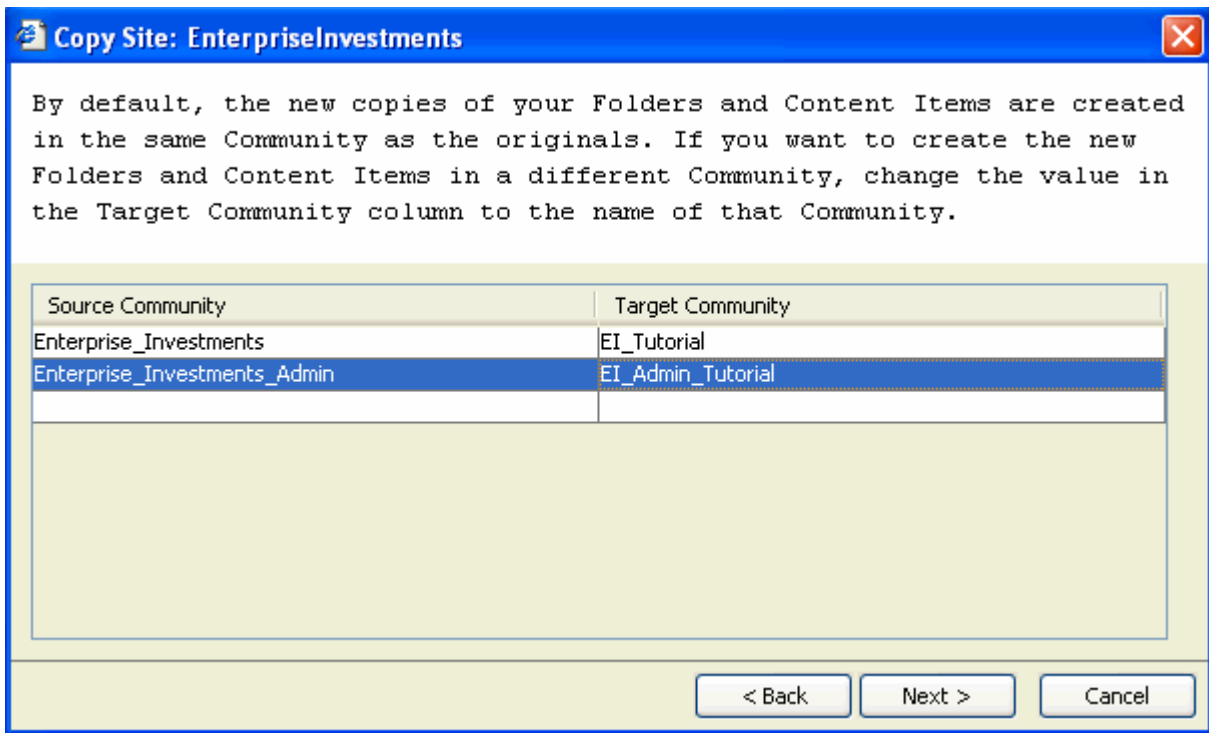
Figure 37: Copy Site Wizard, Map Community Page
