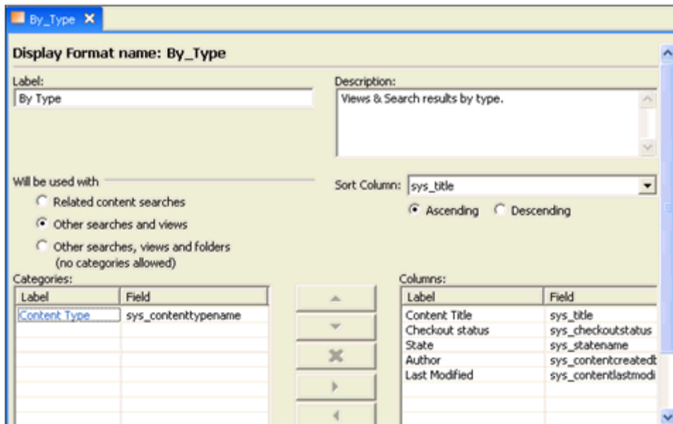
Figure 42: Display Format Editor
