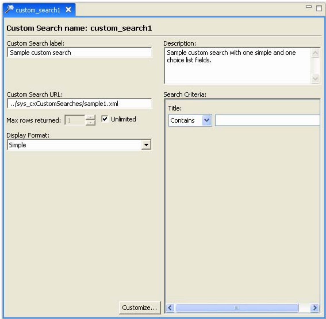
Figure 28: Search Editor, custom searches
